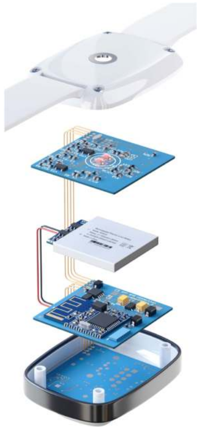
Fig. 1. Exemplary implementation of the wireless portable laser Doppler blood perfusion monitor.
