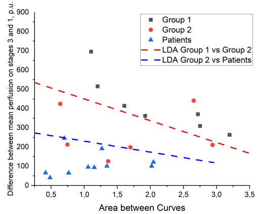
Figure 3. Linear discriminant analysis for groups of volunteers and patients
