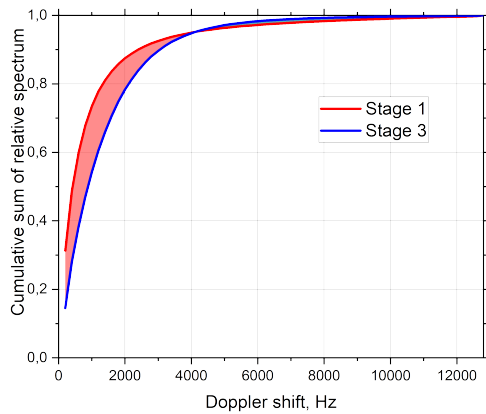
Figure 2. Example of cumulative sum charts for stages 1 and 3 and Area between Curves estimation
